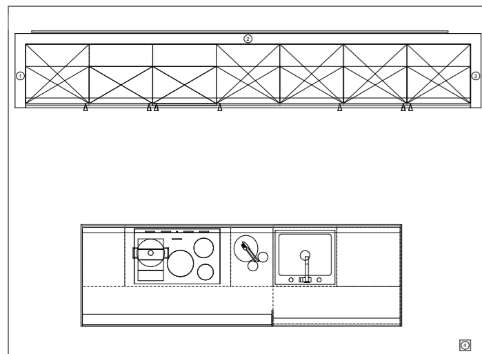
Kojen-Maße | Dimensions | Box | Kooi 4400 mm x 4000 mm
