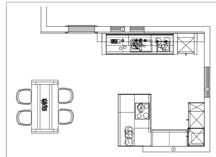
Kojen-Maße | Dimensions | Box | Kooi 4150 mm x 5850 mm
