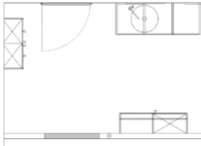
Kojen-Maße | Dimensions | Box | Kooi 2500 mm x 3500 mm
